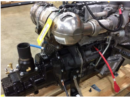
108mm Air End, designed and made in Michigan City, IN
