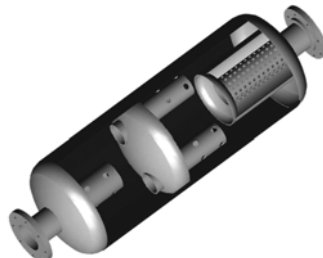
Discharge Silencer
