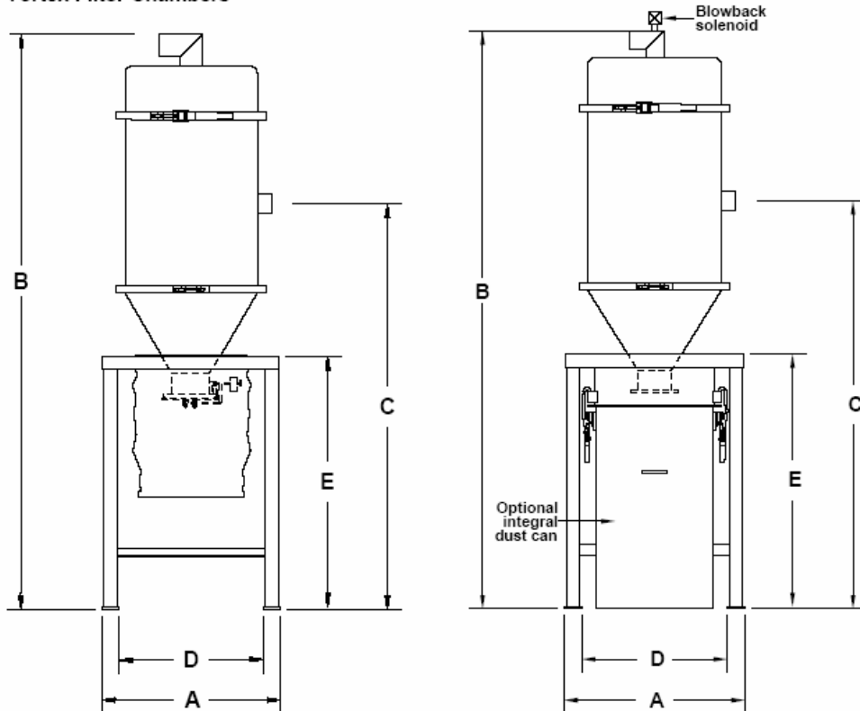
Vortex Filter Chambers
